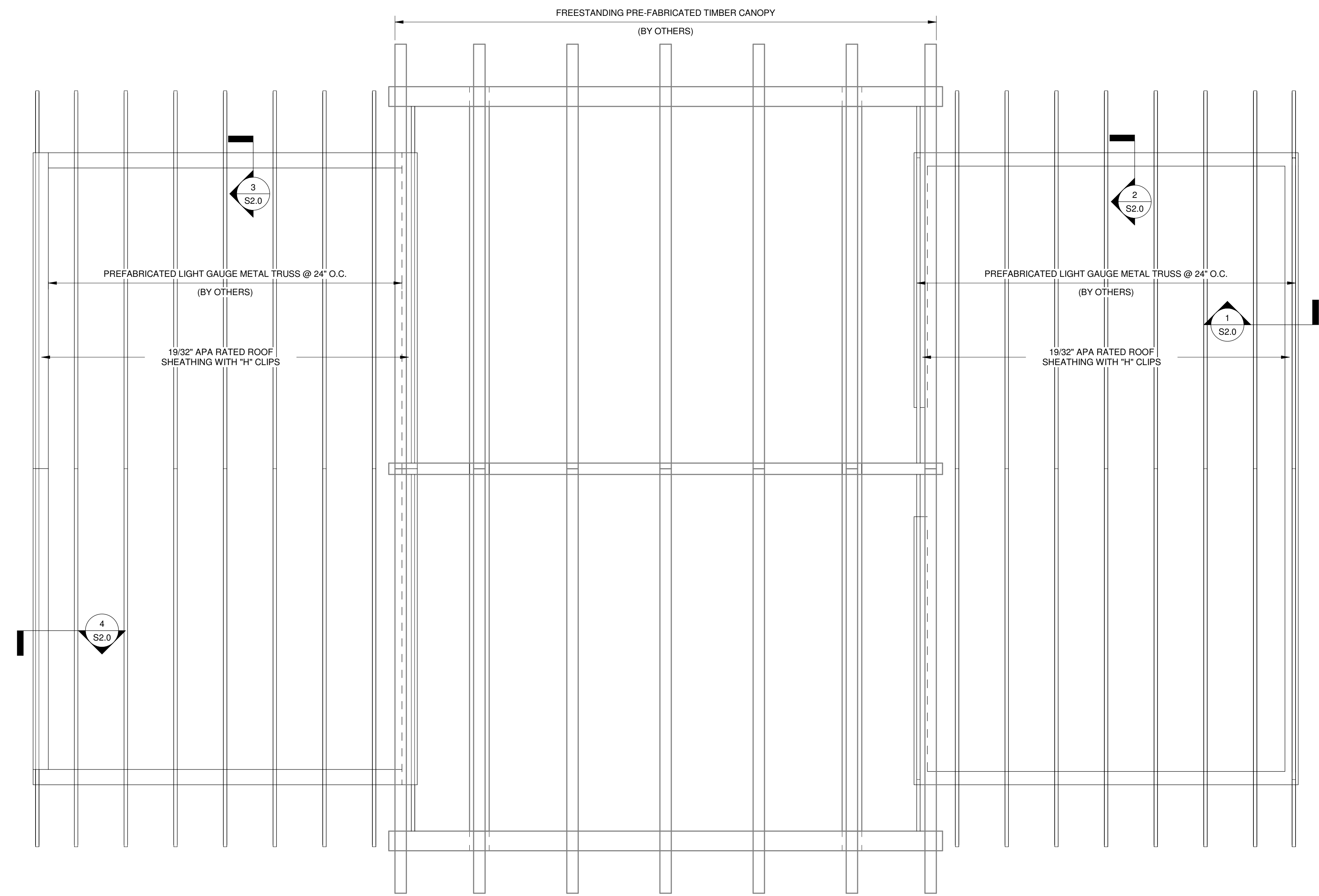
1 FRAMING PLAN S1.1 SCALE: 3/8" = 1'-0"
