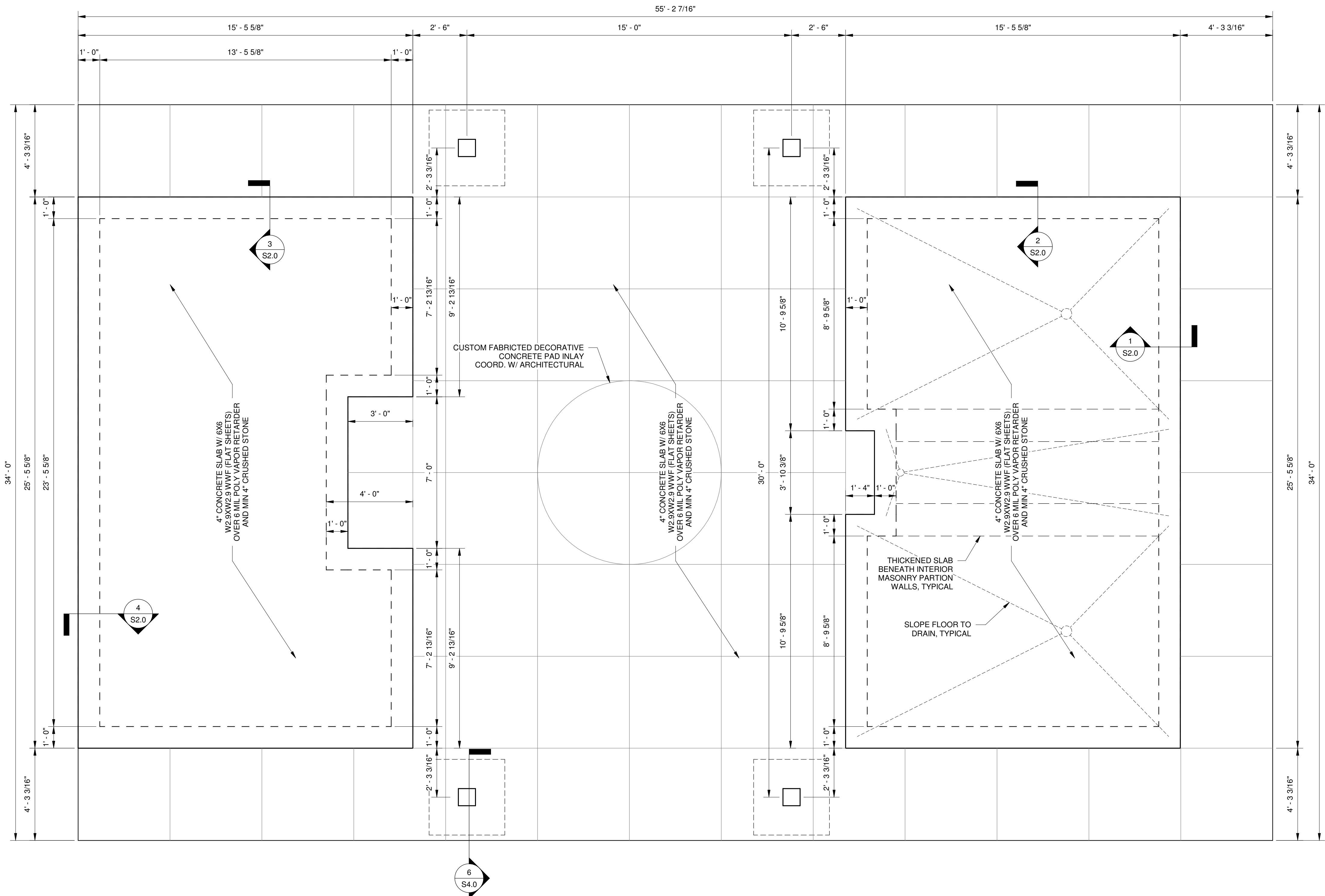
1 S1.0 FOUNDATION & SLAB PLAN SCALE: 3/8" = 1'-0"
