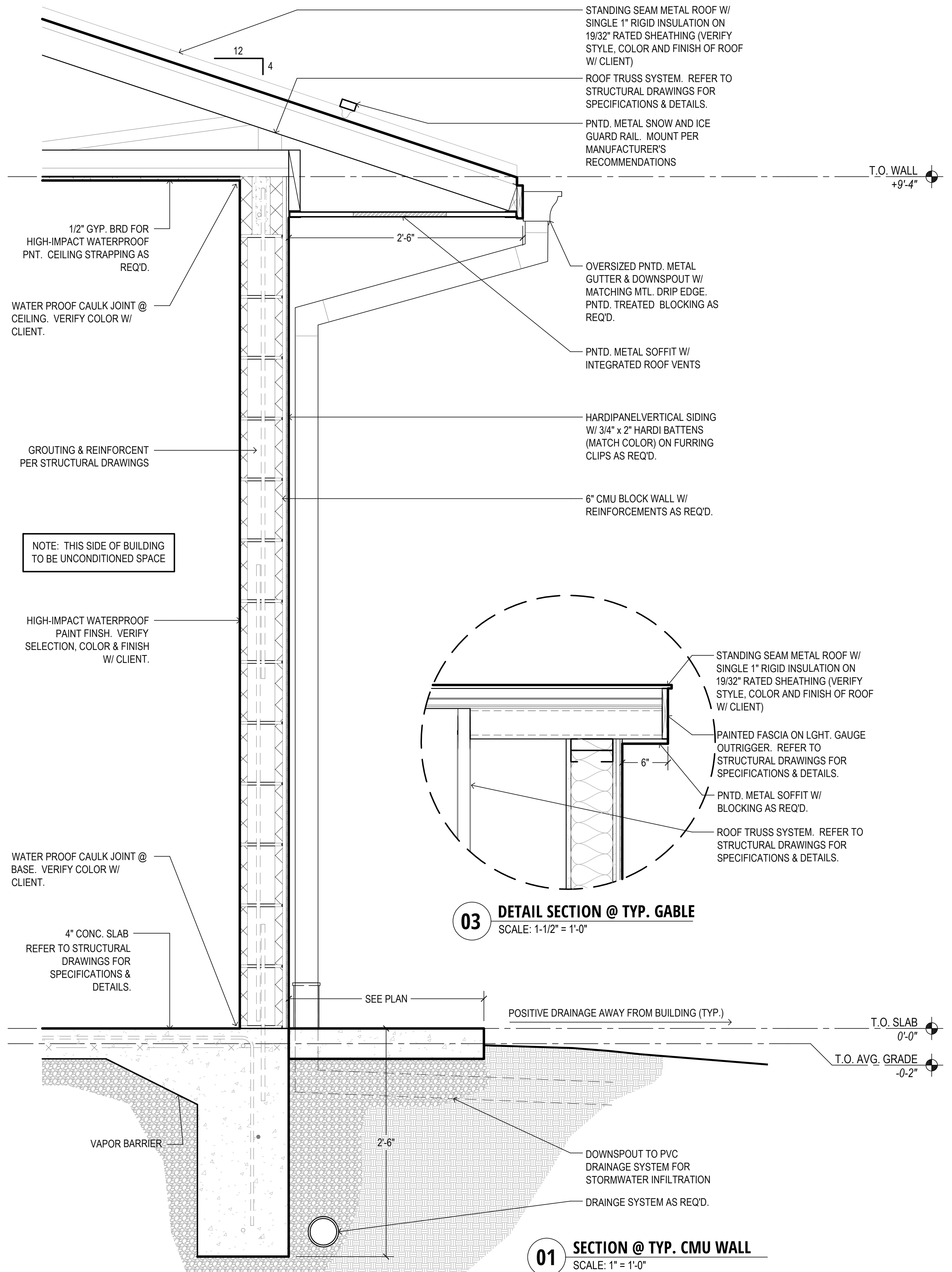
02 SECTION @ TYP. FRAME WALL SCALE: 1-1/2" = 1'-0"
