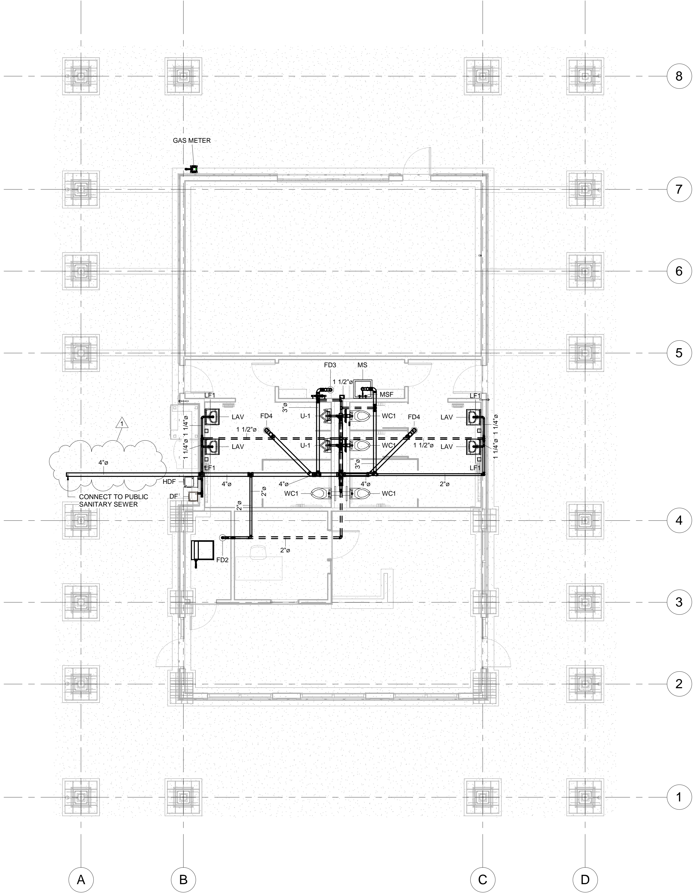
1 1 - SANITARY PIPING SCALE: 3/16" = 1'-0"
