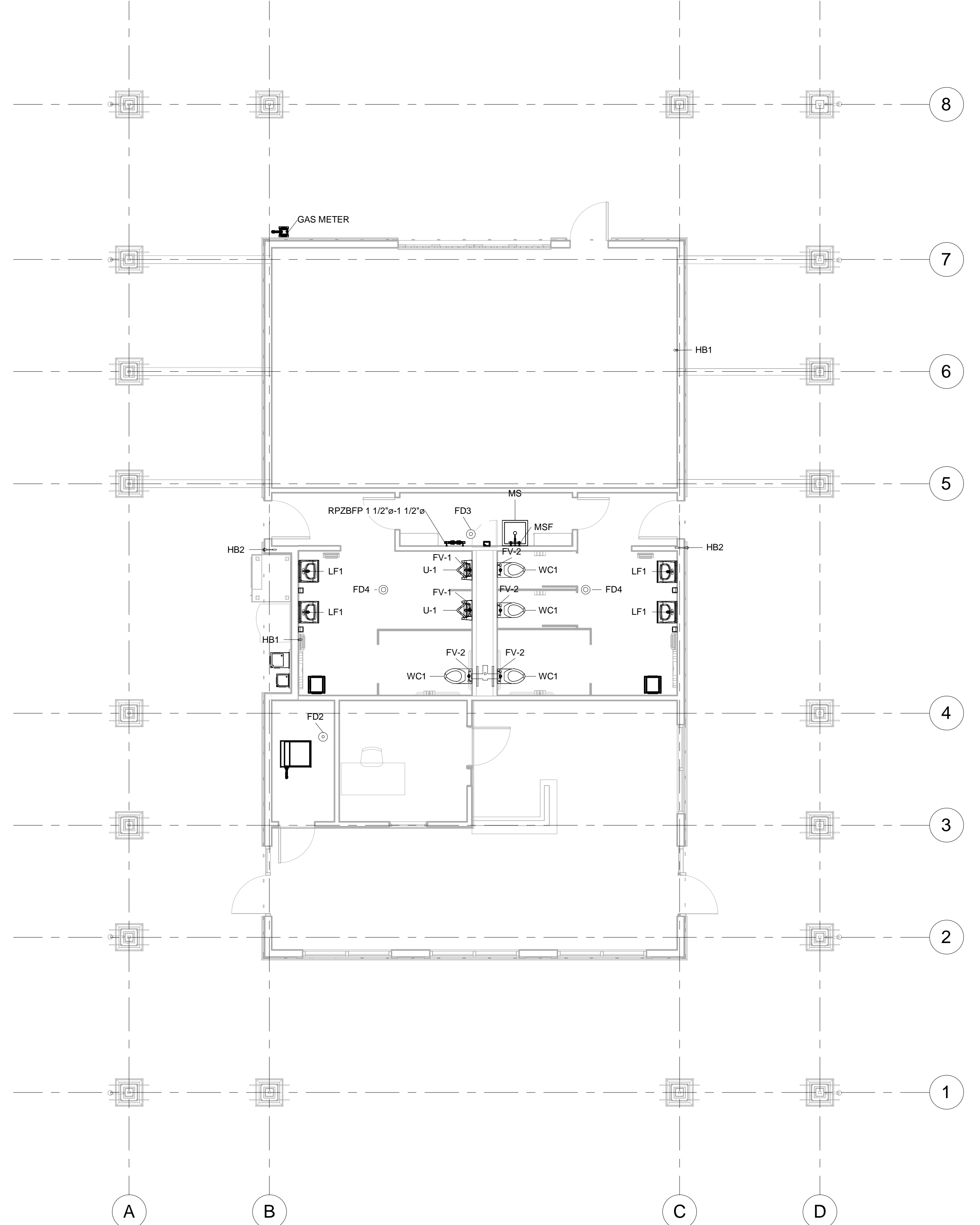
2 1 - DOMESTIC WATER PIPING SCALE: 3/16" = 1'-0"
