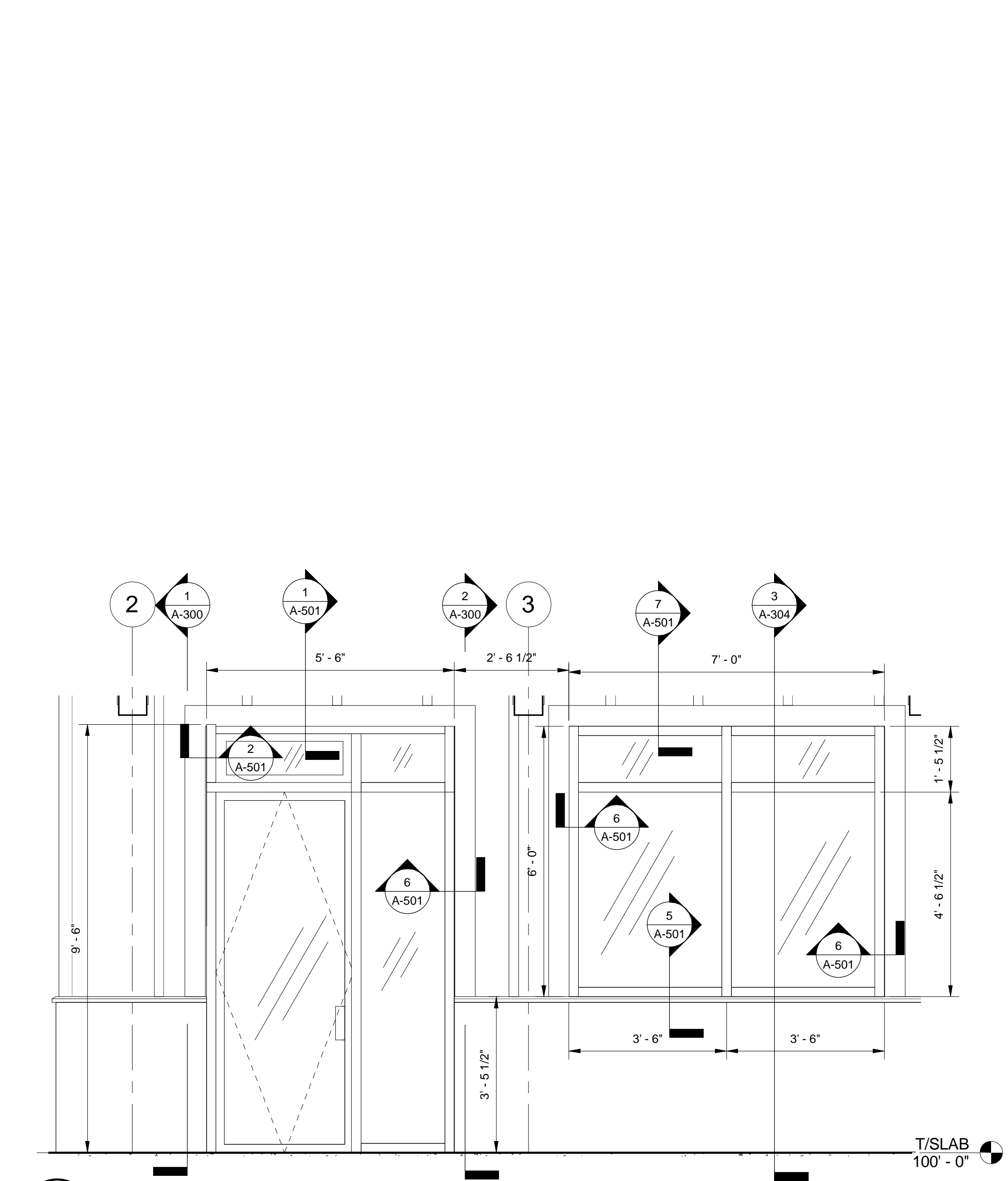
2 SIDE DOOR & WINDOW ELEVATION SCALE: 1/2" = 1'-0"
