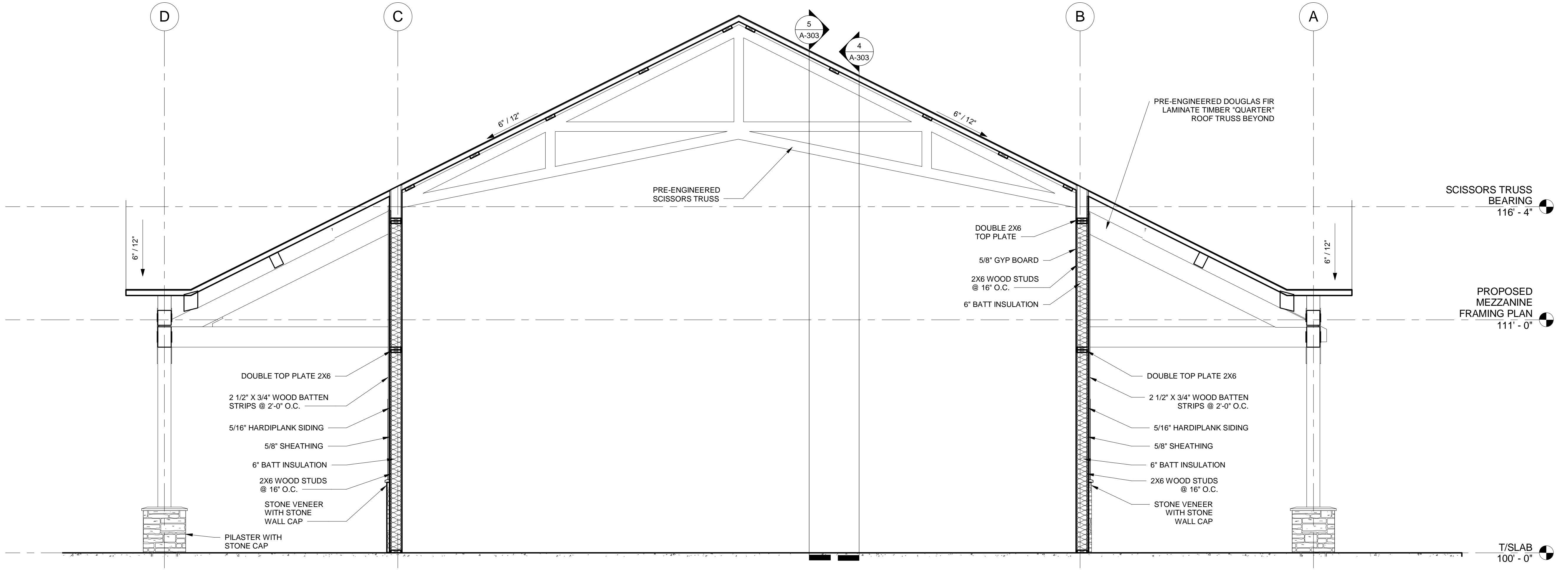
2 BUILDING SECTION WAREHOUSE 1 A-100 SCALE: 3/8" = 1'-0"
