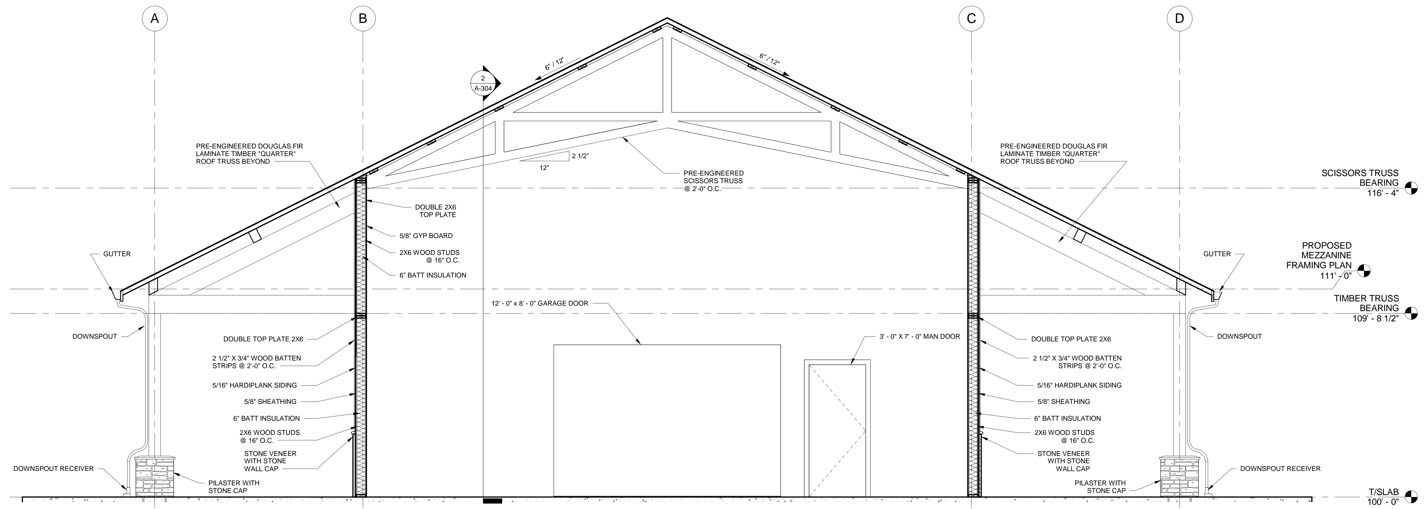
1 BUILDING SECTION WAREHOUSE 2 A-100 SCALE: 3/8" = 1'-0"
