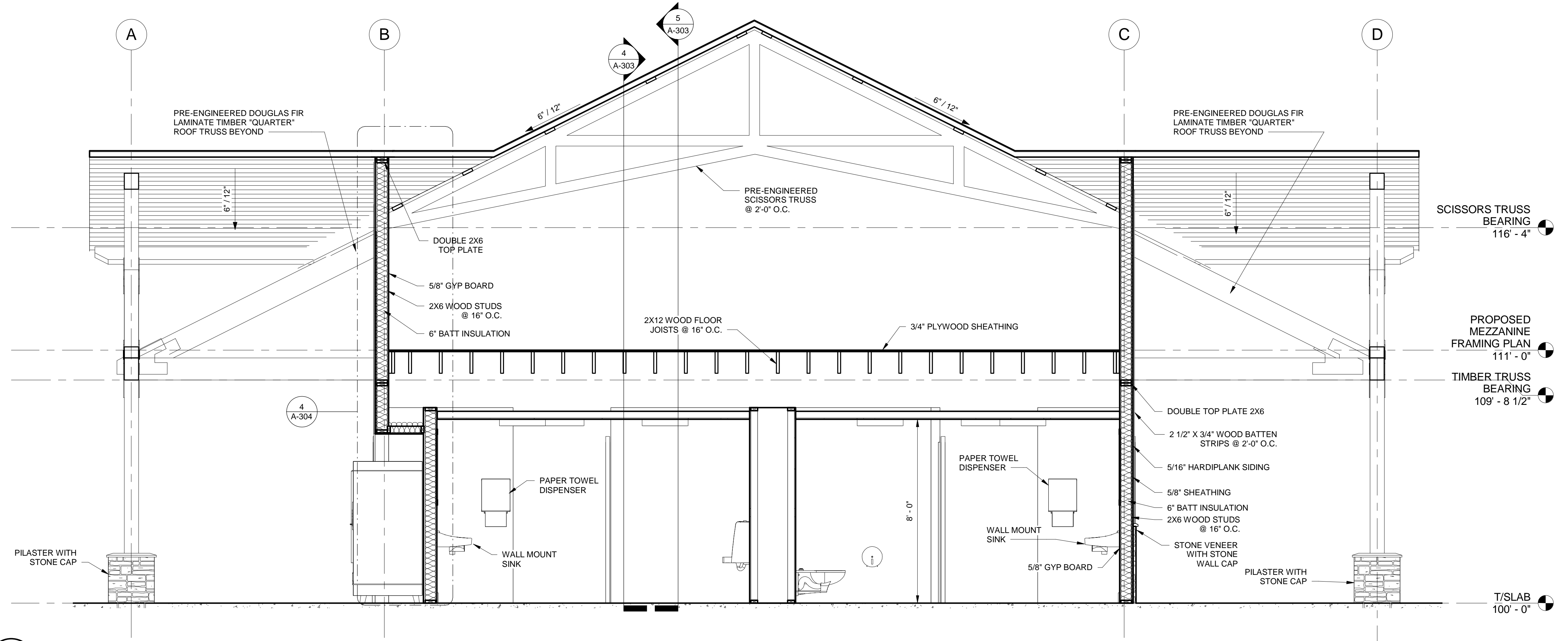
1 BUILDING SECTION RESTROOMS 1 SCALE: 3/8" = 1'-0" A-100
