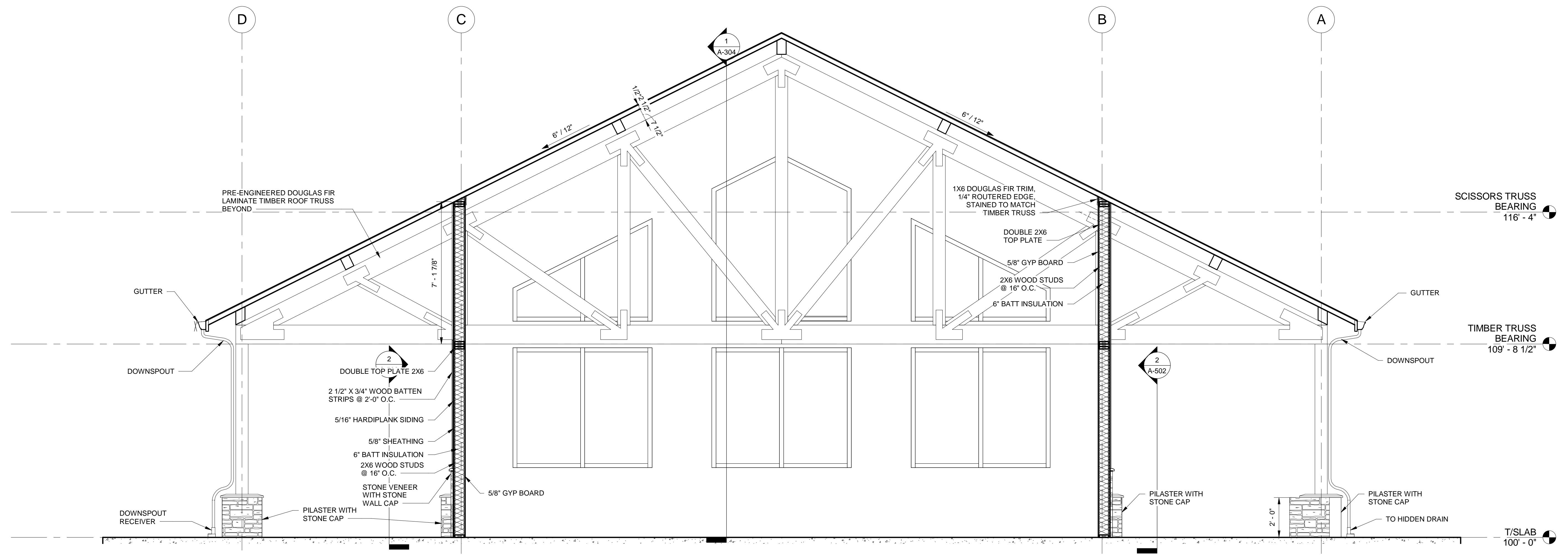
1 BUILDING SECTION LOBBY 1 A-100 SCALE: 3/8" = 1'-0"
