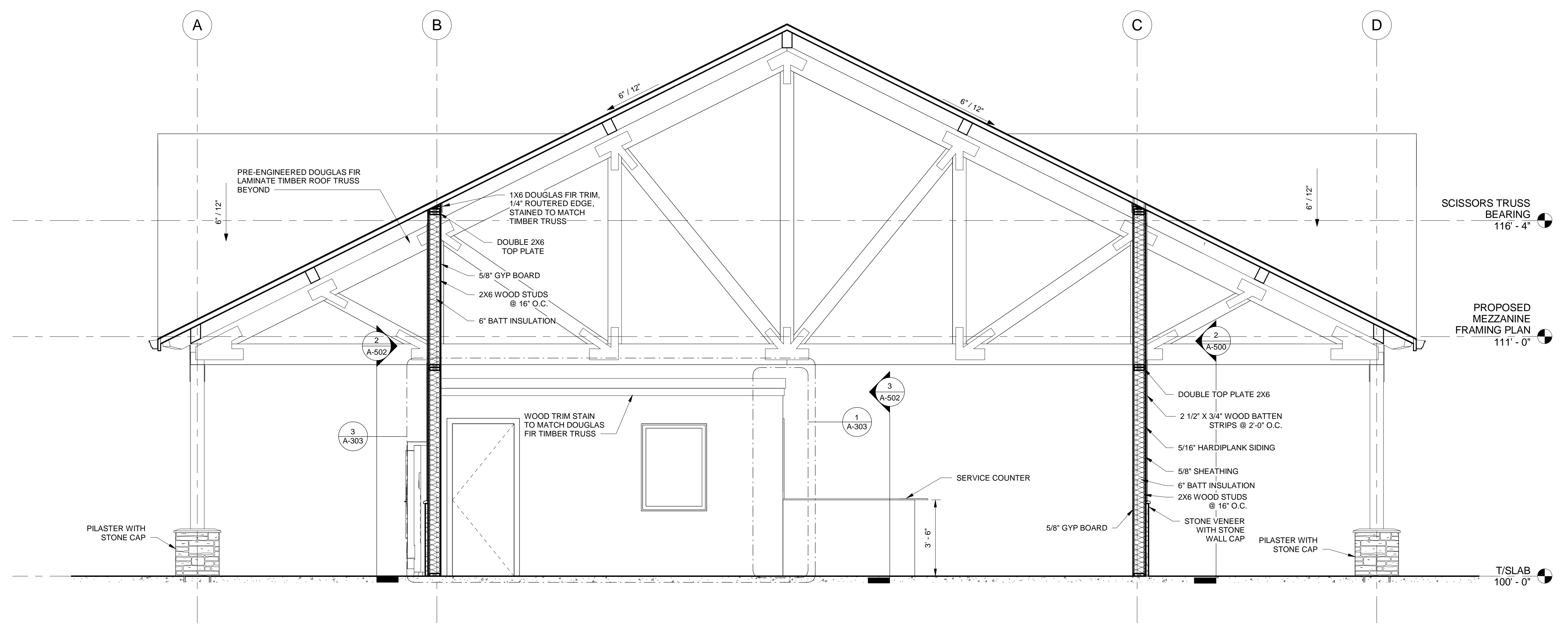
2 BUILDING SECTION LOBBY 2 A-100 SCALE: 3/8" = 1'-0"
