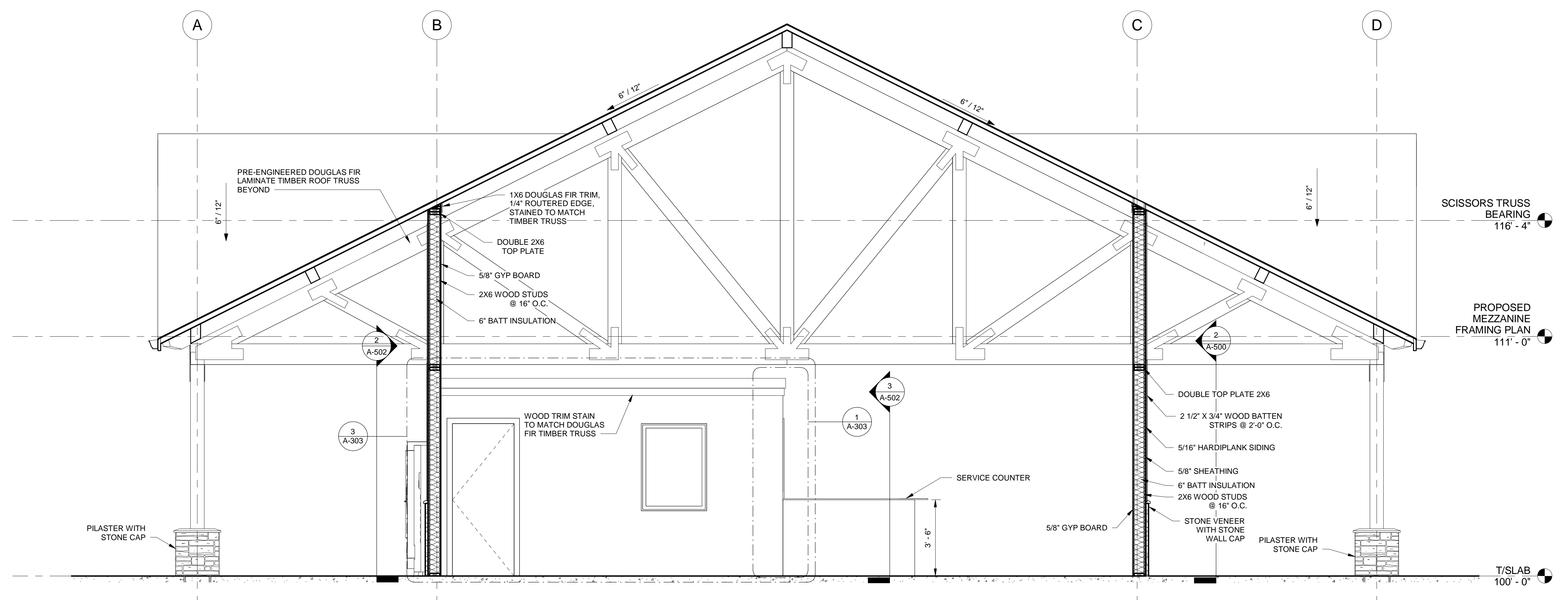
1 BUILDING SECTION LOBBY 1 A-100 SCALE: 3/8" = 1'-0"
