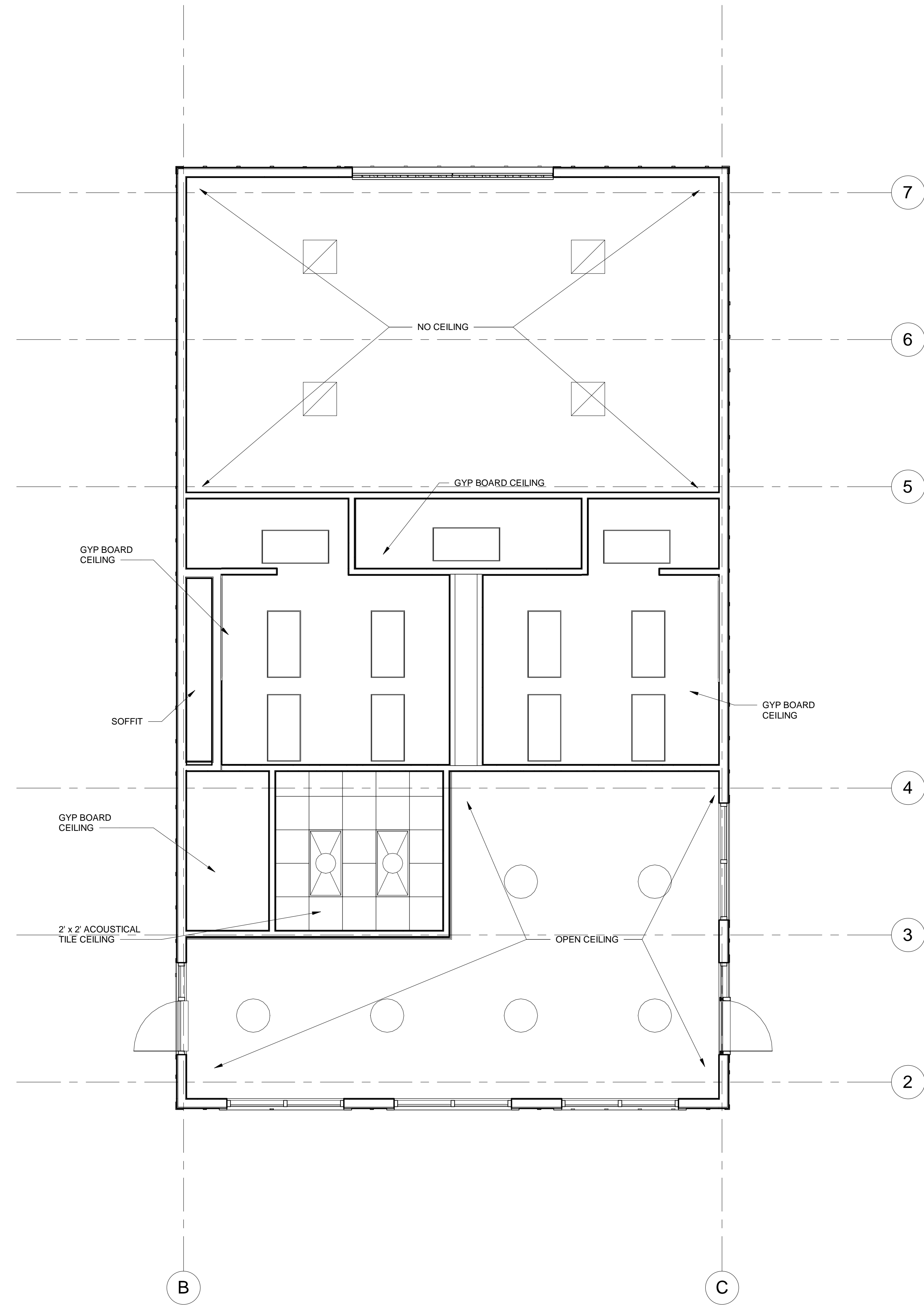
1 REFLECTED CEILING PLAN A-200 SCALE: 1/4" = 1'-0"
